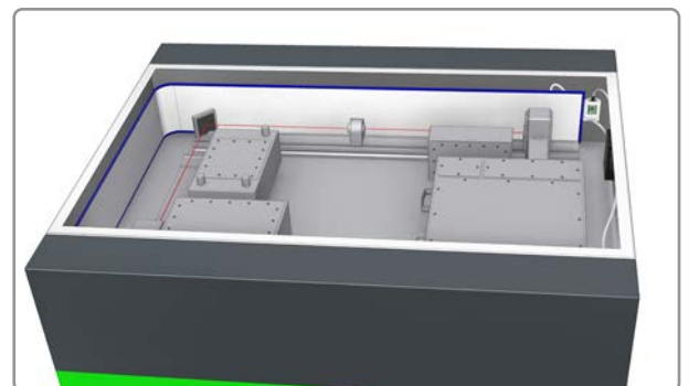
View into the beam path. The active laser protection textile (white) protects the housing locally against escaping of the laser beam.
