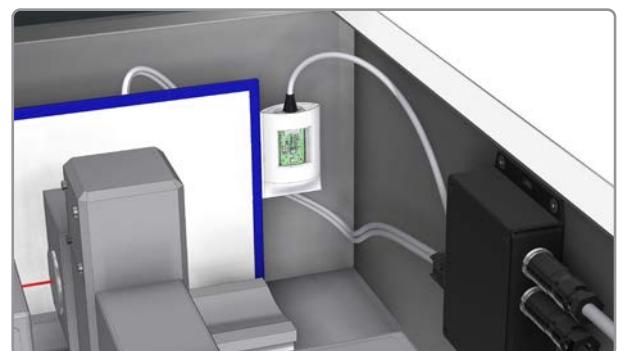
Detailed image of the active laser protection textile and the switch-off electronics.
